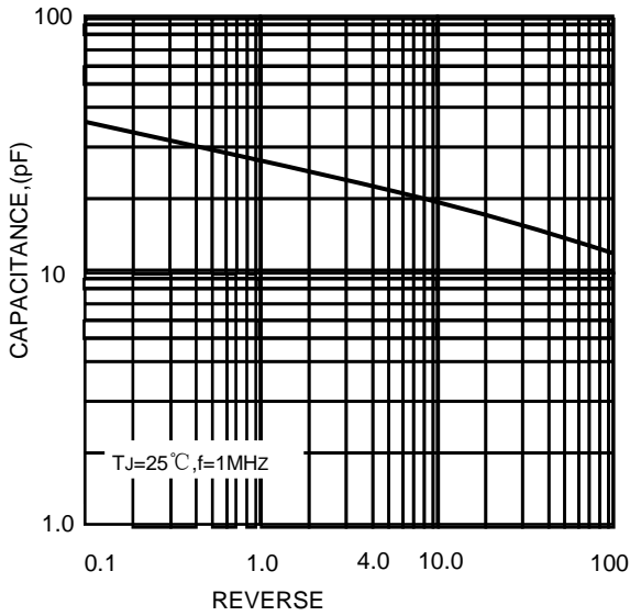
FIG.5-TYPICAL REVERSE
