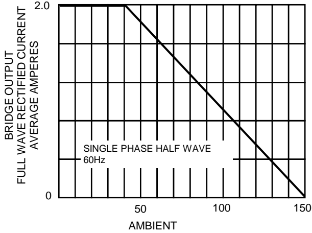
FIG.1-DERATING CURVE FOR
