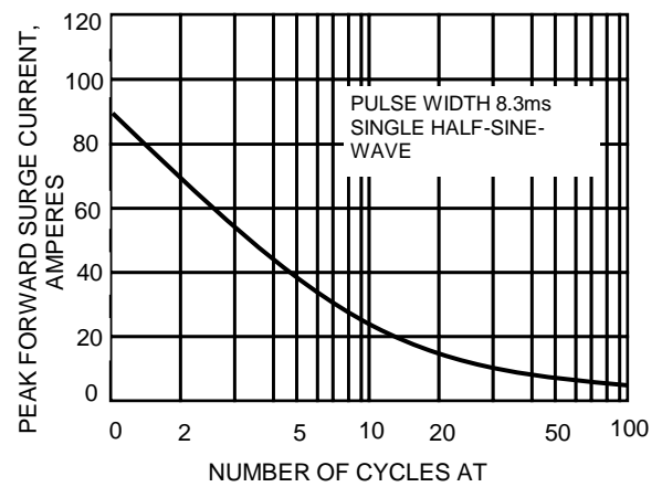
FIG.2-MAXIMUM NON-REPETITIVE SURNGE
